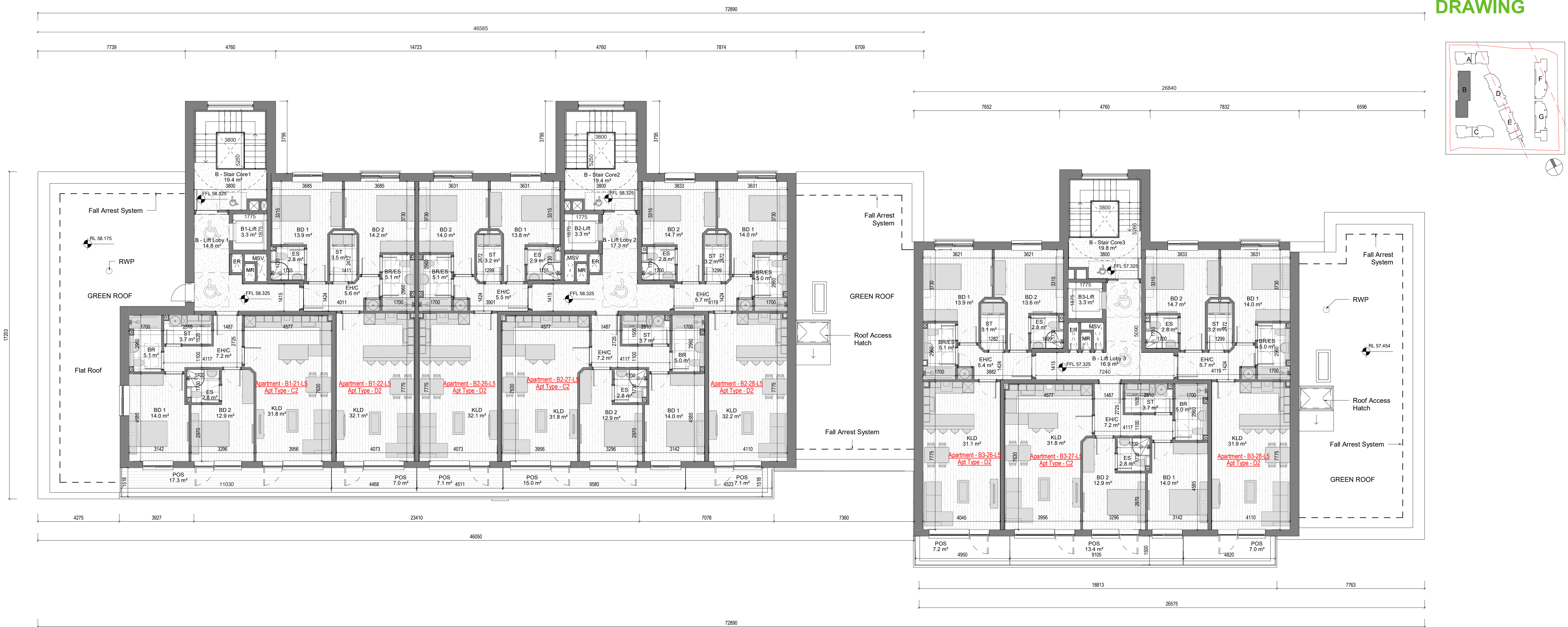
1 GA - Fifth Floor Plan 1 : 100
